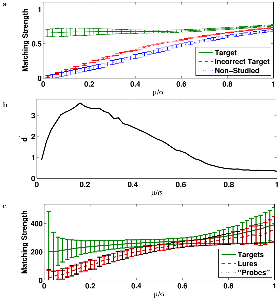
Figure 6. Simulation of the realistic spiking model. (a) Tested with cued recall, plotting matching strength (normalized dot product) relative to strength of the correct target. (b,c) Item memory retrieved from the spiking-neuron Association Model with constant-current input. Means and standard deviations of strengths for targets (right-hand items within studied pairs), lures and “probes” (left-hand items within studied pairs) are depicted in (c). Horizontal axes ( \mu/\sigma ) are aligned for comparison across panels. Note that for the simulation, \mu/\sigma refers to the theoretical, not actual values observable in firing rates, which are truncated at zero.
