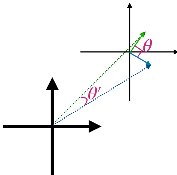
Figure 1. Schematic depiction of the effect of features values having a non-zero mean. Two vectors, depicted in blue and green solid lines, respectively, start out orthogonal relative the origin (thin axis lines). Thus, the angle between them, \theta = 90^\circ . When a constant value is added to all cells of the vectors (in this simple example, only two dimensions each), the geometric interpretation is that the origin is shifted (thick axis lines). The new vectors (darker, dotted lines) now have a much smaller angle, \theta' , between them. Because cued recall starts with, mathematically, a dot product between the probe item and the memory matrix, the addition of a bias has the effect of cueing, to some degree (depending on the magnitude of the bias itself), all other associations.
