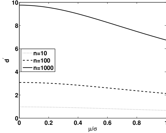
Figure 2. Analytic solution for the Item Memory model: d' for list length 10, as a function \mu (relative to \sigma ), for three example values of vector dimensionality ( n ).
