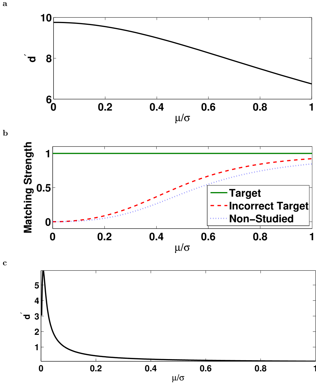
Figure 3. Analytic solution for the Item Model, Equation 11, with L = 10 , n = 1000 (a); cued recall of the Association Model (b), where matching strength (dot product of retrieved vector, \mathbf{g}_r , with candidate response item vectors) is plotted relative to strength of the correct target (Equations 15–17), and item memory retrieved from the Association Model (Equations 30–31) (c). The horizontal axes ( \mu/\sigma ) are aligned for comparison across panels.
