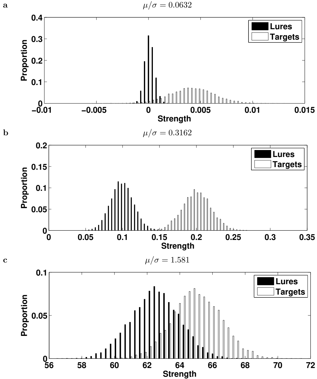
Figure 4. Probability distributions of matching strengths for targets and lures, from the numerical simulation with n = 1000 , L = 10 , averaged across 1000 simulated lists. a) \mu = 0.002 , d' = 2.66 . b) \mu = 0.01 , d' = 5.59 , c) \mu = 0.05 , d' = 1.65 .
